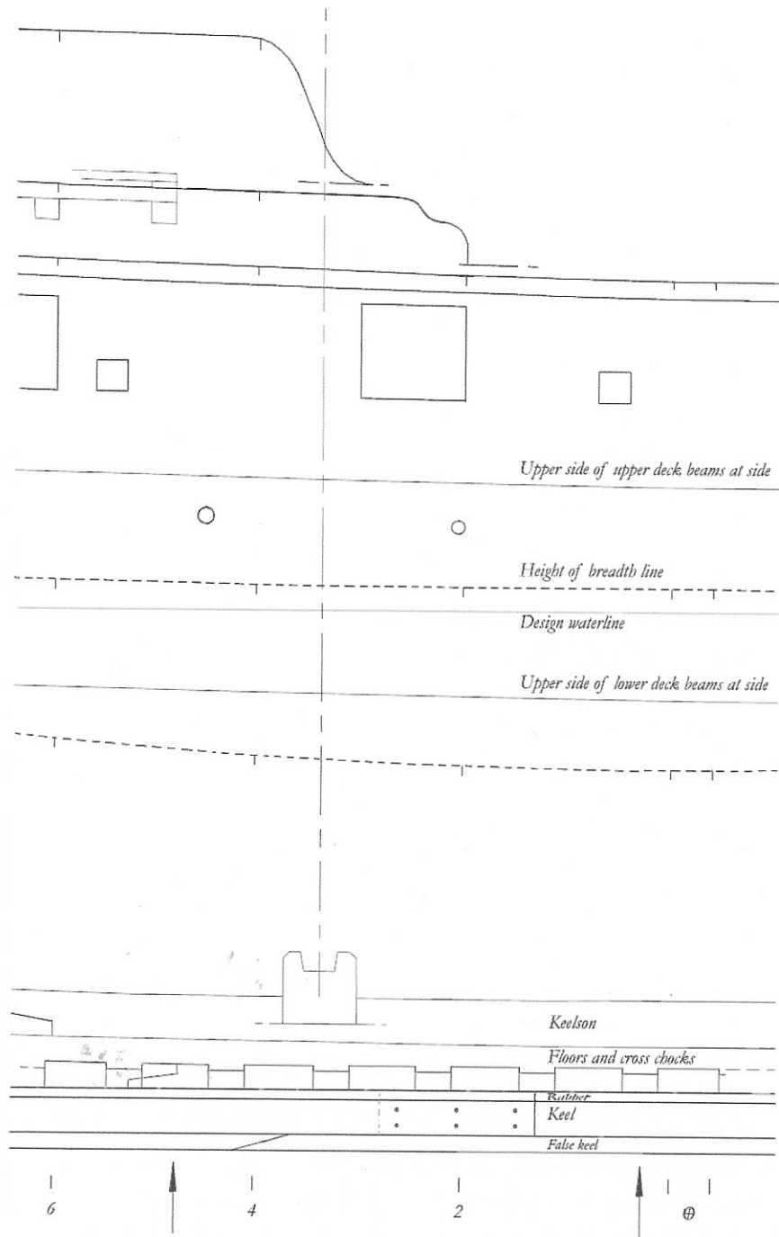
From the Admiralty Models sheer plan based on the sheer & profile of Echo, 1781. ©David Antscherl, 2010, 2012
